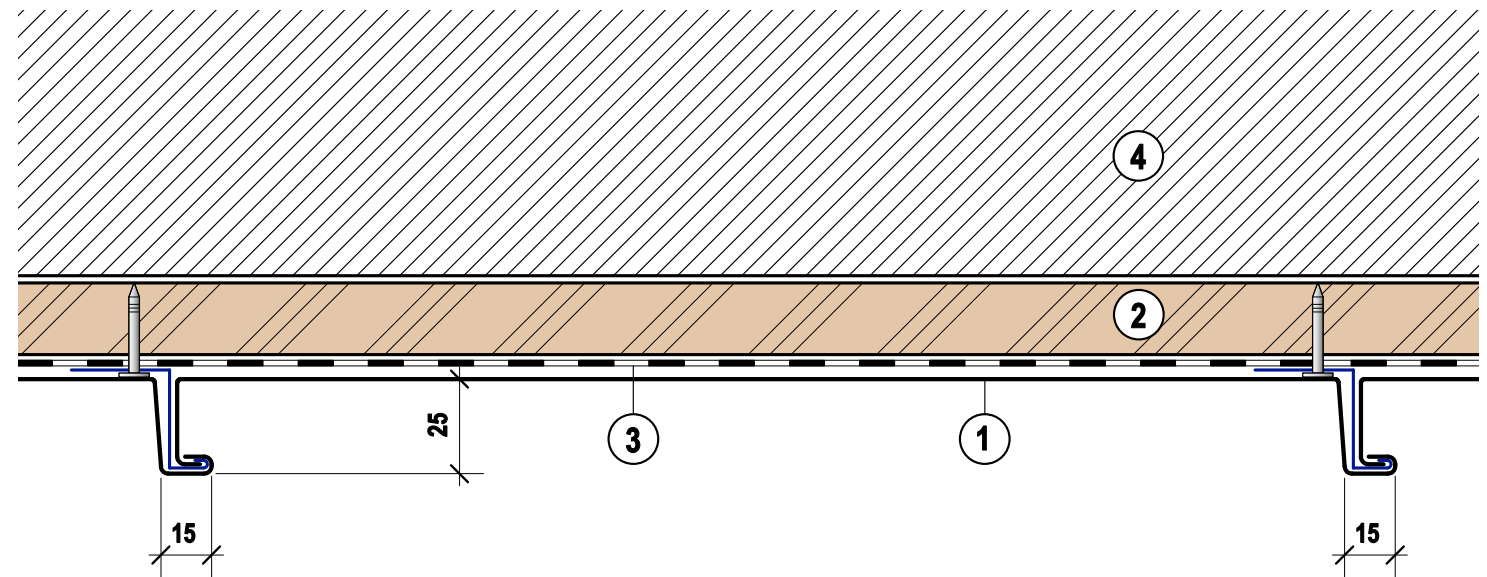
TYPICAL HORIZONTAL SECTION
